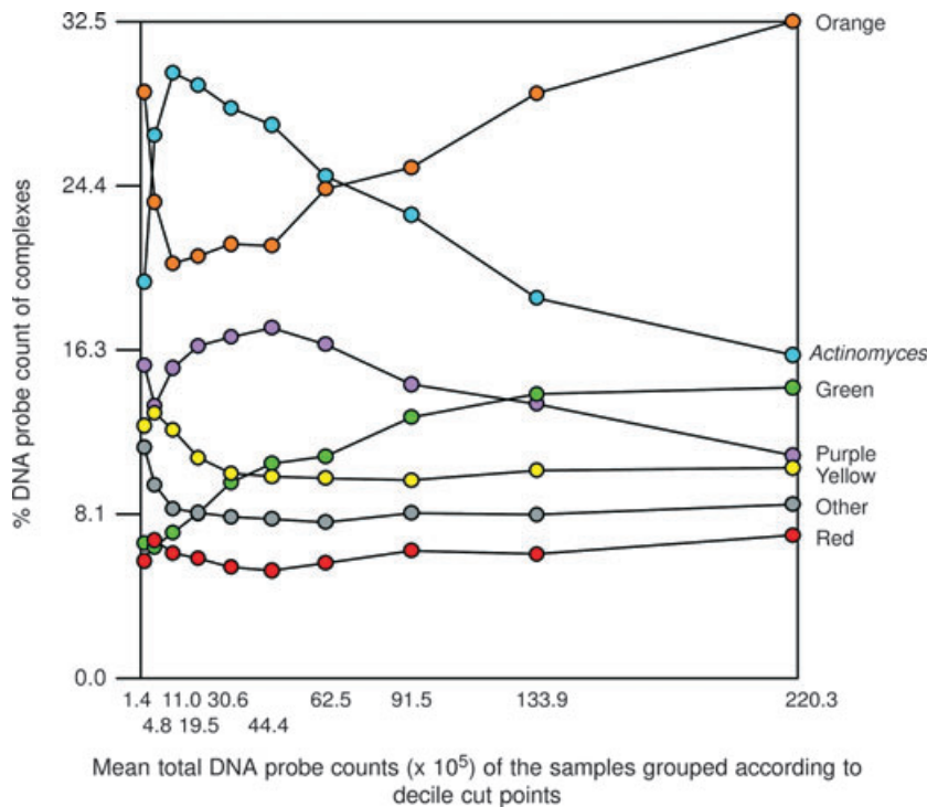
Fig. 4. Plot of the total mean proportions of each of the seven supragingival complexes described by Haffajee et al. (136). The samples were divided, according to total-DNA probe counts, into 10 groups using the 10, 20, 30, 40, 50, 60, 70, 80 and 90th percentiles of the total counts as cut-off points. The x-axis values represent the mean values for total-DNA probe counts of each group and the y-axis represents the sum of the proportions comprised by the species in each microbial complex. Printed with permission from Haffajee et al. (139).
