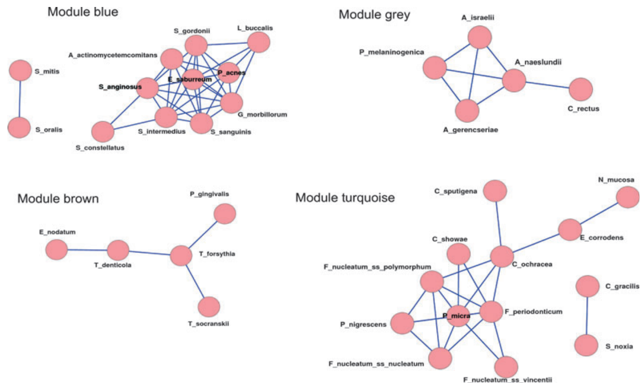
Fig. 14. Weighted correlation network analysis results based on data obtained using checkerboard DNA–DNA hybridization. The images show the Cytoscape representation of the correlation networks for the four modules identified by weighted correlation network analysis. Checkerboard analysis was performed for 40 species of oral bac-
