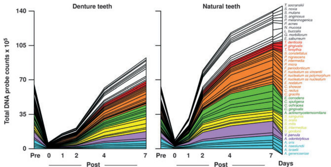
Fig. 6. Cumulative mean counts ( \times 10^5 ) of 41 bacterial species in samples taken from 55 subjects with natural teeth and from 62 subjects with full-mouth dentures. Samples were taken before professional removal of the dental biofilms (Pre), immediately after cleaning (time 0) and after 1, 2, 4 and 7 days of redevelopment (Post). The subjects refrained from oral-hygiene procedures for the 7-day test period. Samples were removed before, and immediately after cleaning from the mesio-buccal aspect of each natural tooth (excluding third molars) and from each denture tooth. In addition, samples were obtained
