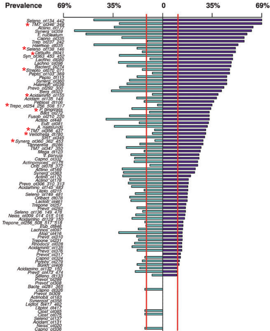
Fig. 15. Prevalence of uncultured/unnamed taxa and 'reference' culturable species ( Fusobacterium nucleatum , Porphyromonas gingivalis , Veillonella parvula and Actinomyces naeslundii ) examined in samples from periodontally healthy individuals (aqua) ( n = 8 ) and from patients
