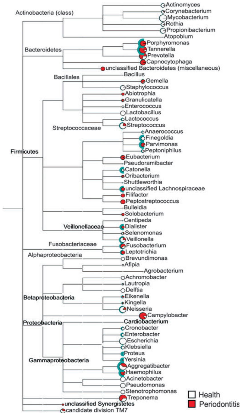
Fig. 21. Metatranscriptomics from pooled samples from 74 sites from a periodontally healthy subject (no bleeding on probing, no gingival redness and pocket depth <2 mm) and pooled samples from 27 diseased sites from a subject with untreated chronic periodontitis (pocket depth >6 mm with bleeding on probing). Phylogenetic assignments of metatranscriptomic reads were performed using software for analyzing metagenomes [MEtaGenome ANalyzer (MEGAN)]. Illumina sequences from metatranscriptomic analysis were assigned to phylogenetic groups using BLAT results. Numbers of reads were normalized to database size, which are represented by different sizes of the pie charts. Reads from healthy patients are in white and reads from patients with periodontal disease are in red. Green semicircles represent the statistical significance of the differences after Holm–Bonferroni correction. The taxa identified were clustered according to phyla and genus.
