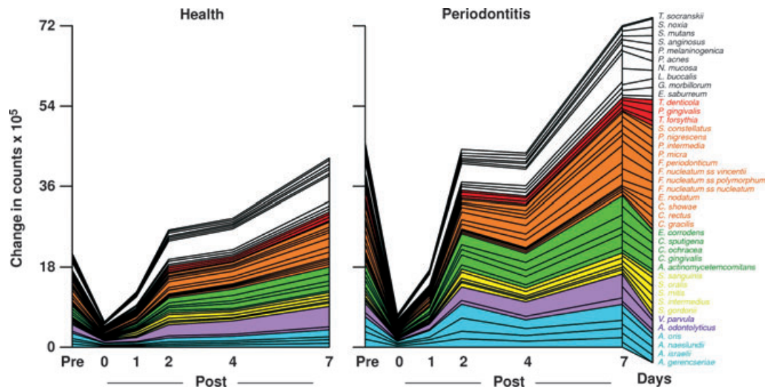
Fig. 7. Cumulative mean counts ( \times 10^5 ) of 41 bacterial species in subgingival samples taken from 38 periodontally healthy subjects and from 17 subjects with periodontitis before professional removal of the dental biofilms (Pre), immediately after cleaning (time 0) and after 1, 2, 4 and 7 days of redevelopment (Post). Species counts in the samples were averaged within each subject
