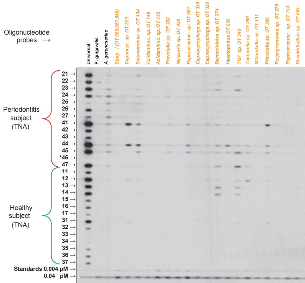
Fig. 13. An RNA-oligonucleotide quantification technique membrane showing hybridization of clinical samples with oligonucleotide probes. Probes for uncultured/unnamed species ('orange' group of bacteria) are listed across the top. Each horizontal lane represents the total nucleic acids
