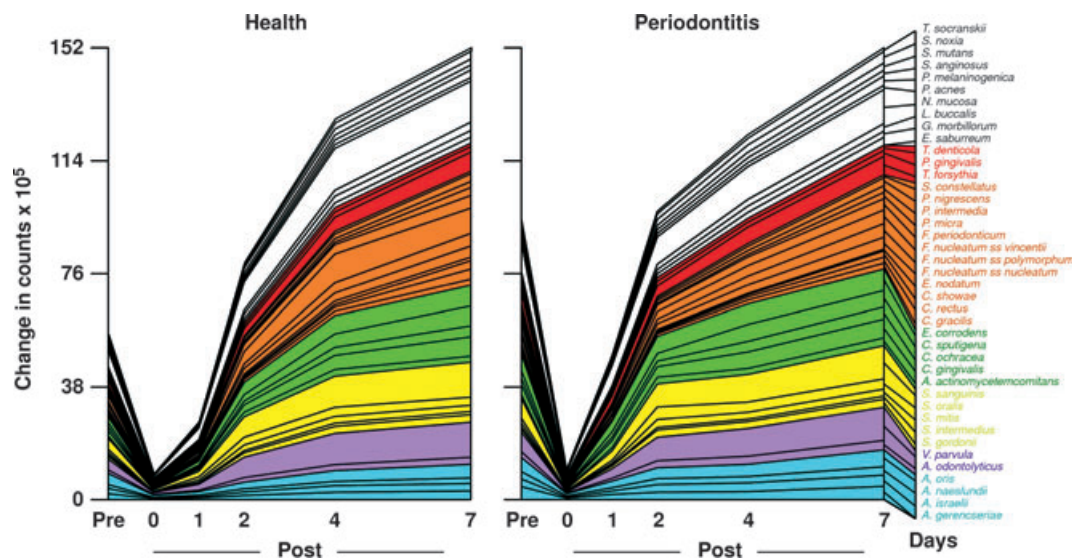
Fig. 1. Cumulative mean counts ( \times 10^5 ) of 41 bacterial species in supragingival samples taken from 38 periodontally healthy subjects and from 17 subjects with periodontitis before professional removal of the dental biofilms (Pre), immediately after cleaning (time 0) and after 1, 2, 4 and 7 days of redevelopment (Post). The subjects refrained from oral-hygiene procedures for the 7-day test period. Samples were removed, pre-cleaning and immediately post-cleaning, from the mesio-buccal aspect of each tooth (excluding third molars). In addition, supragingival samples were obtained from up to seven
