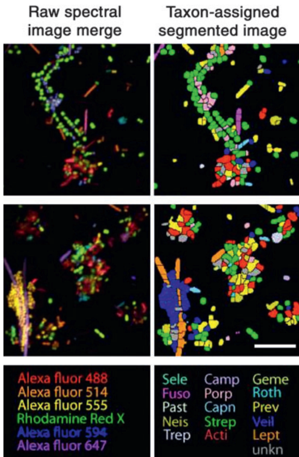
Fig. 18. Representative detail images of combinatorial labeling and spectral imaging–fluorescence in-situ hybridization-labeled semidispersed human dental plaque. The color in the raw spectral images represents a merge of six different fluorophore channels. The color in the segmented image represents one of 15 taxa. Scale bar = 10 \mu m. Printed with permission from Valm et al. (375).
