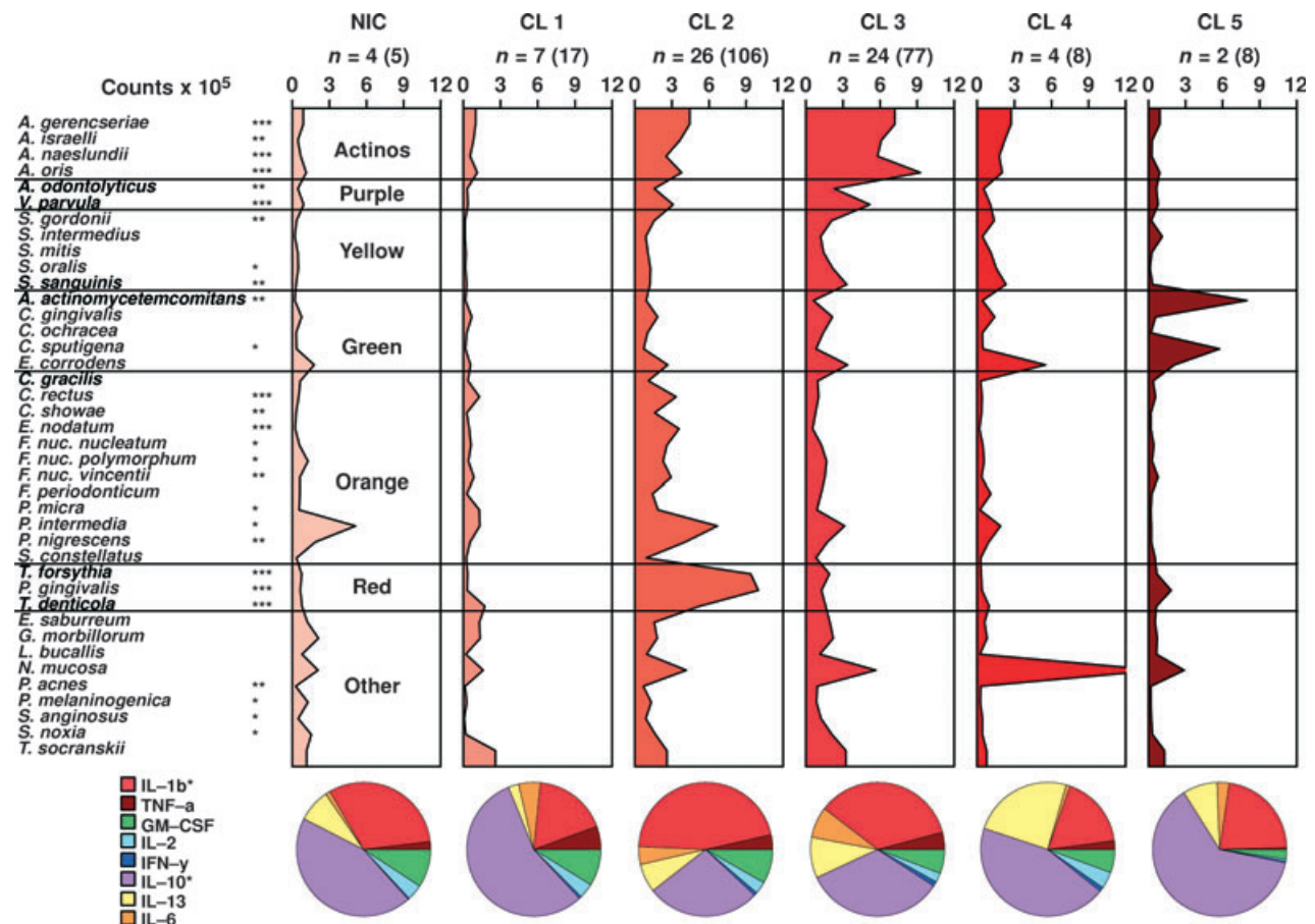
Fig. 19. Mean counts (×10 5 ) of subgingival taxa in the clusters and not-in-cluster group detected in 31 subjects with generalized aggressive periodontitis. The counts of 40 subgingival species were measured at each of up to 14 sites in each subject and were employed in a cluster analysis using the chord coefficient and an average unweighted linkage sort. Five clusters (CL1–CL5) were formed at >33% similarity. Four subjects presented at least one site with a microbial profile that did not fit any cluster (NIC). The numbers above each panel represent the number of subjects with at least one site with the microbial profile that defined that cluster. The numbers in parentheses represent the total number of sites in each cluster. After the clusters were identified, data were averaged within a subject and then averaged across subjects in each cluster group separately. The numbers above each panel represent the number
